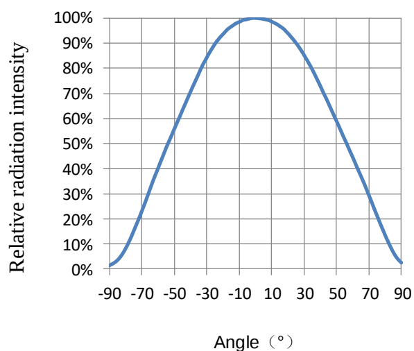
Figure7. Relative radiation intensity vs. Angle
