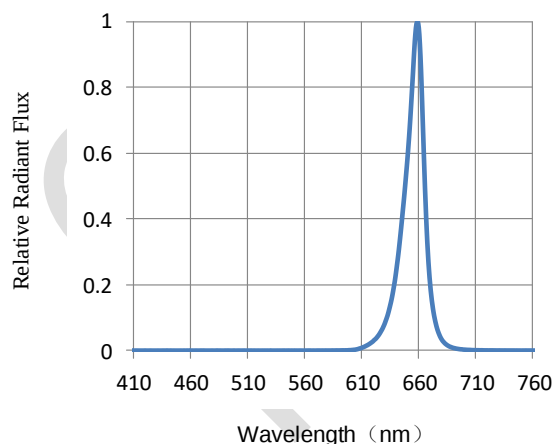
Figure 5. Relative Radiant Flux vs. Wavelength
